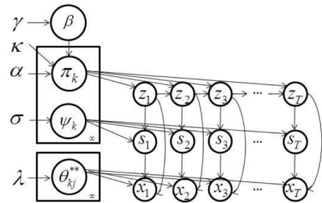
Figure 2. A graphical representation of an HDP-HMM is shown that integrates a mixture distribution model with an infinite HMM.
