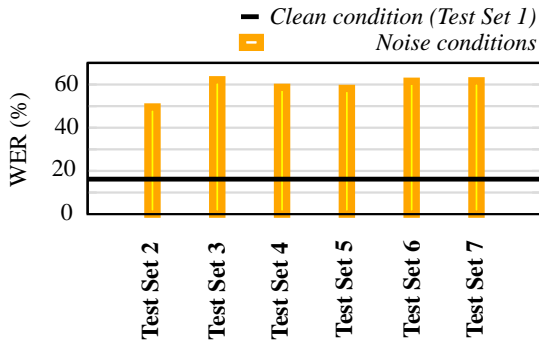
Figure 3: A comparison of the WER for six noise conditions at 8 kHz on TS1.
