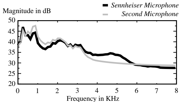
Figure 2: The Sennheiser close-talking microphone preserves frequencies above 3.5 KHz better on the average than the variety of microphones used on the second channel.
