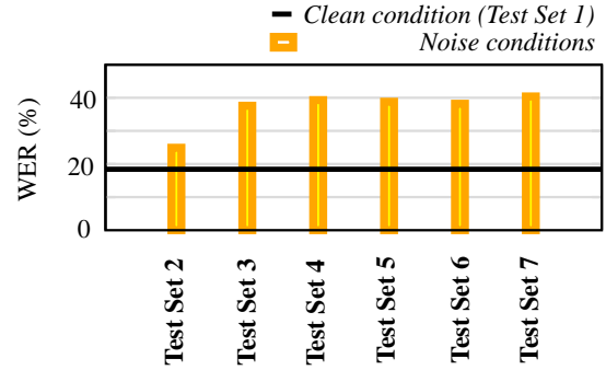
Figure 4: A comparison of the WER for six noise conditions at 8 kHz on TS2.
