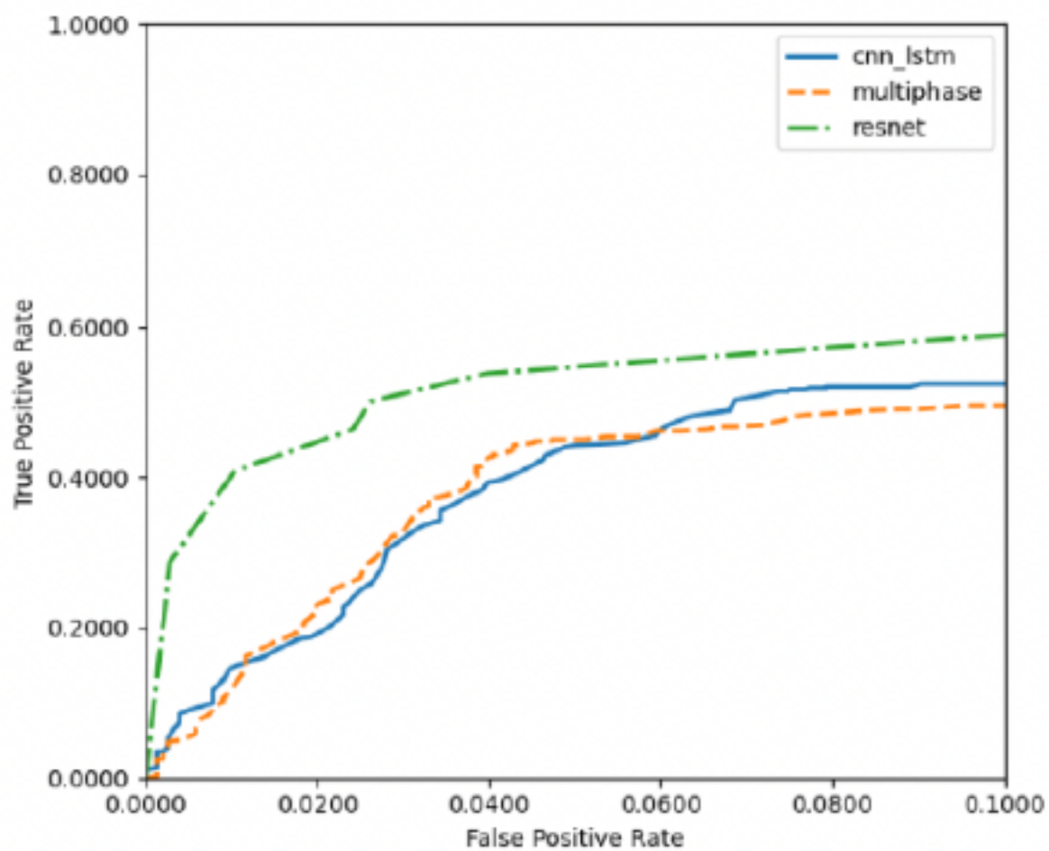
Figure 8. An ROC comparison on the evaluation dataset
