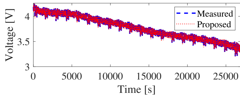
Figure 7.9. Voltage results on UDDS test data.
