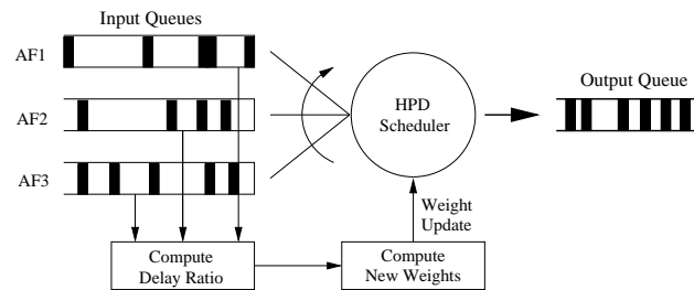
Figure 3.1 Adaptive HPD
