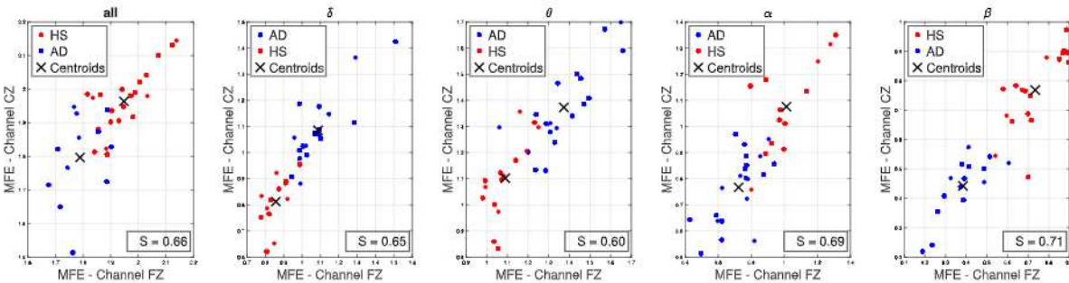
Fig. 6. K-means clustering results for each EEG frequency band. For visualization clarity, each dot represents the average MFE value on scale factors.
