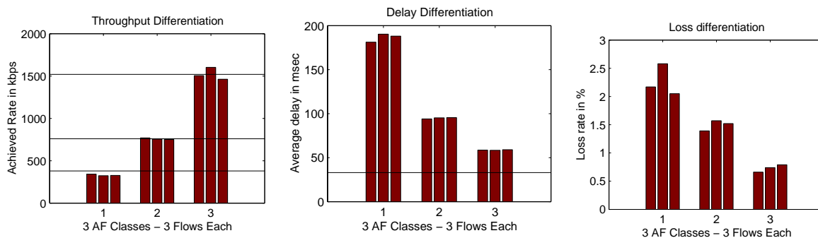
Figure 8. AHPD and CRED. Exponential traffic over SACK.
