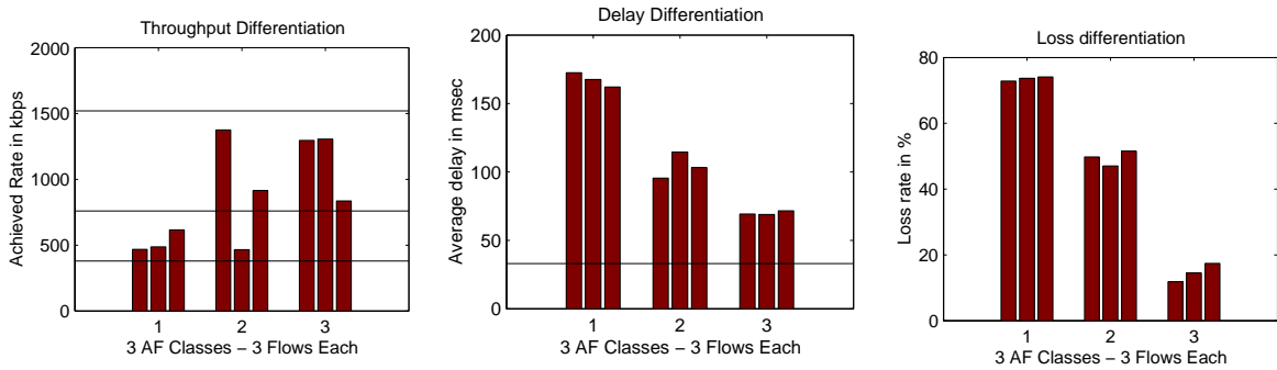
Figure 12. Original HPD: Pareto over UDP.
