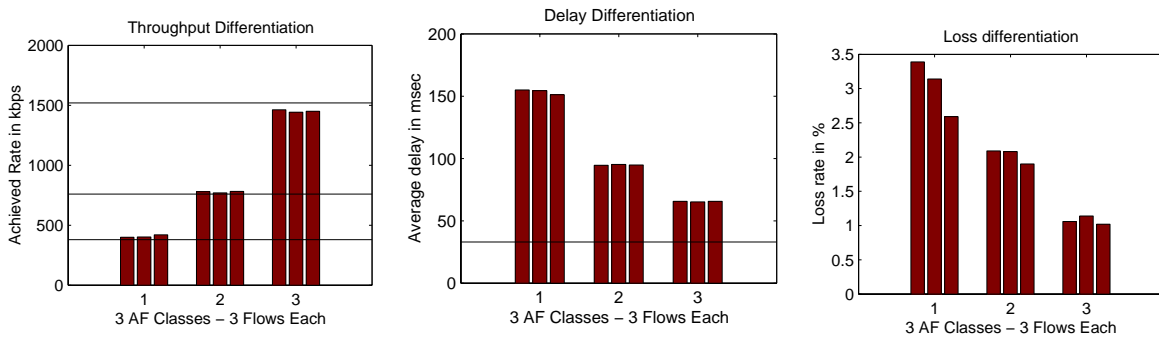
Figure 4. Original HPD and RIO. FTP over TCP SACK. Bottleneck = 8 Mbps.
