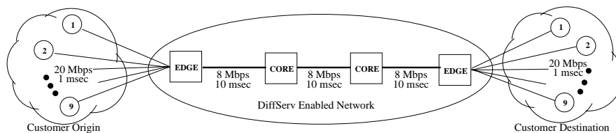
Figure 2. Block diagram of the simulation topology used to evaluate the performance of AHPD.
