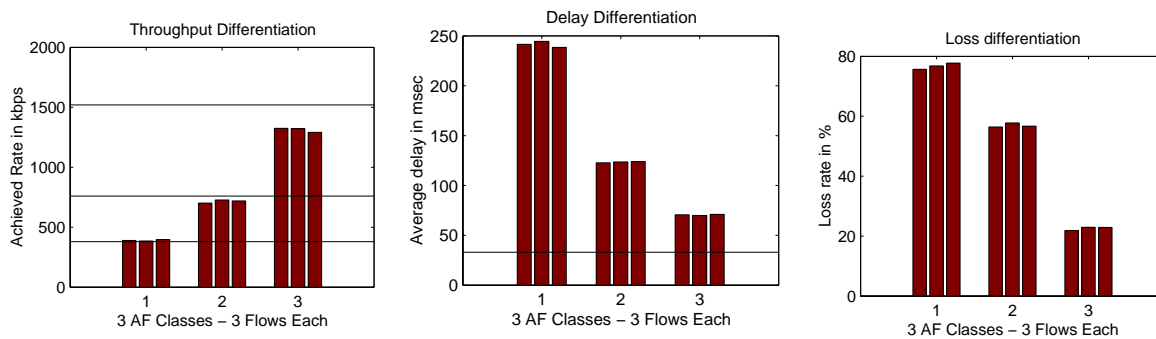
Figure 9. AHPD and CRED. Exponential traffic over UDP.
