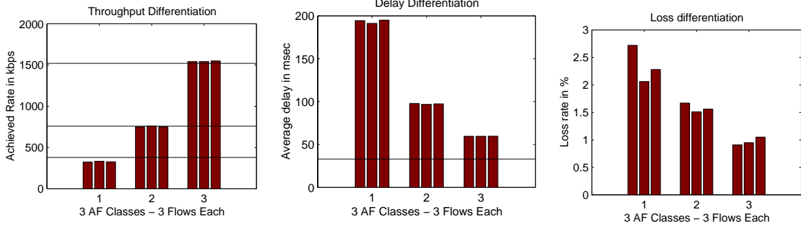
Figure 3. AHPD and CRED. FTP over TCP SACK. Bottleneck = 8 Mbps.
