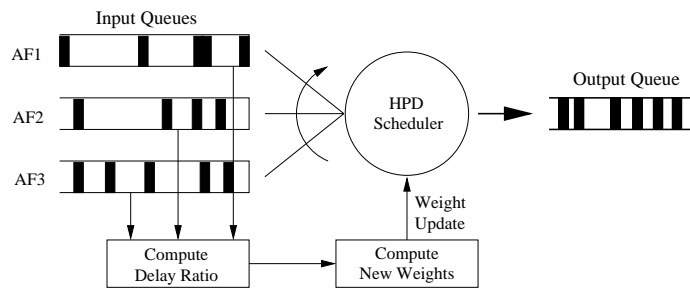
Figure 1. Block diagram describing the operation of Adaptive HPD.
