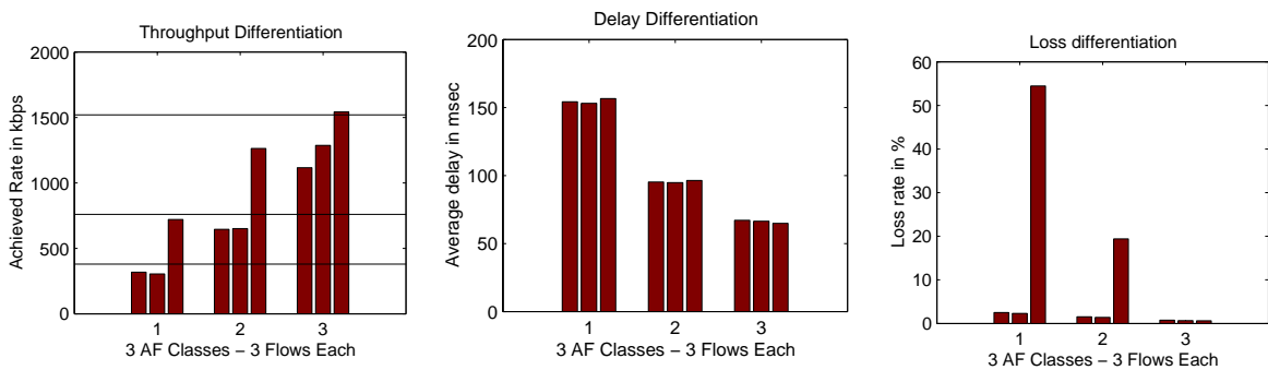
Figure 14. Original HPD: CBR/UDP and Pareto/TCP.
