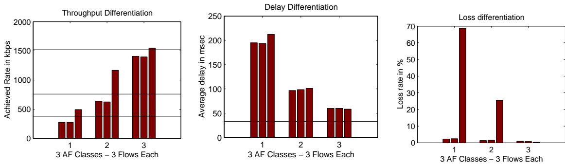
Figure 13. AHPD and CRED: CBR/UDP and Pareto/TCP.
