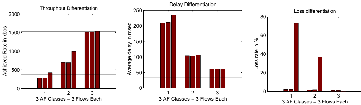
Figure 6. AHPD and CRED. Experiment with CBR. One flows in each class is CBR over UDP. Rest FTP/SACK
