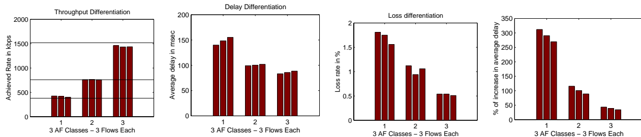
Figure 16. AHPD and CRED. Flows with Different RTT.
