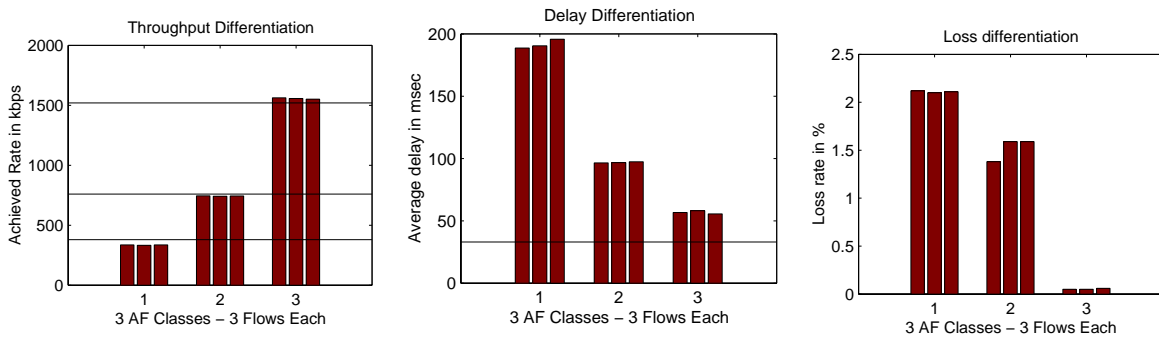
Figure 5. AHPD and CRED. All 9 flows are CBR over SACK.
