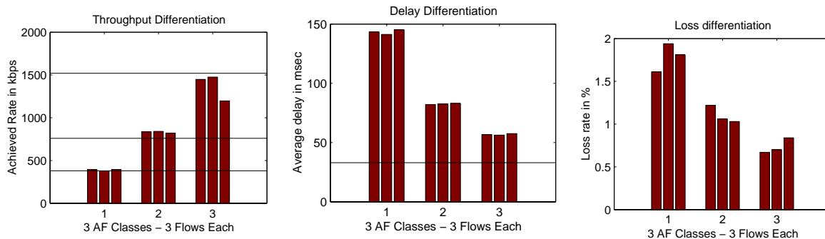
Figure 10. AHPD and CRED: Pareto over SACK.
