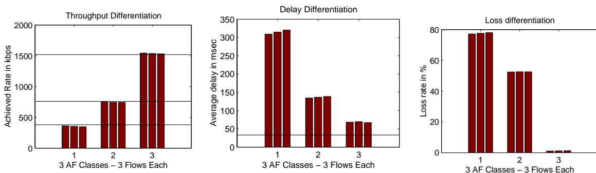
Figure 7. AHPD and CRED. All 9 flows are CBR/UDP
