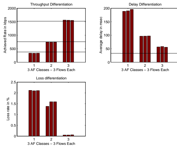
Figure 5. AHPD and CRED. All 9 flows are CBR over SACK
