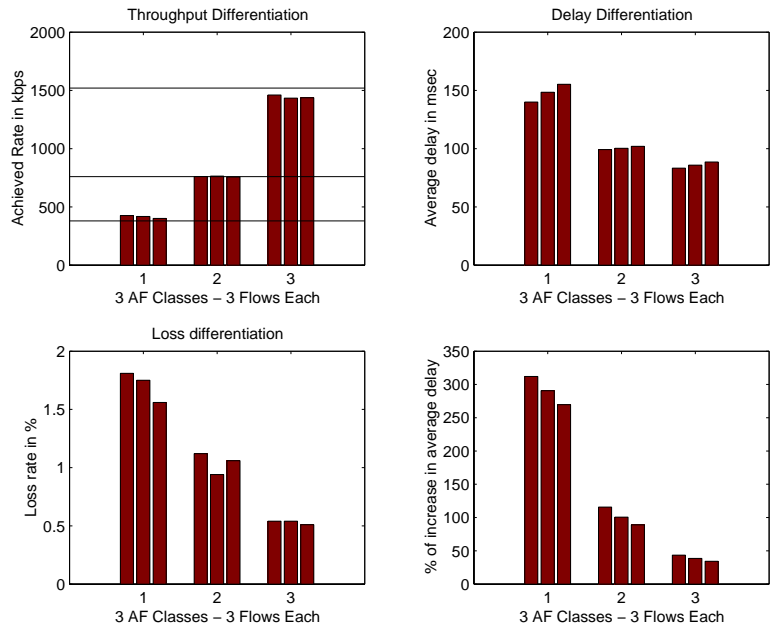
Figure 16. AHPD and CRED. Flows with Different RTT
