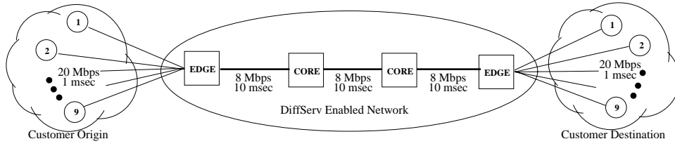
Figure 2. Simulation Topology
