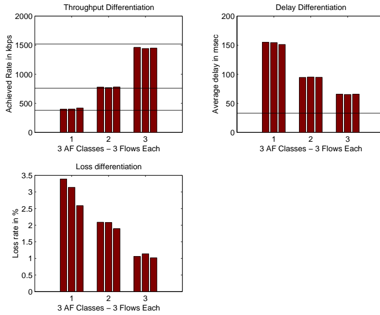
Figure 4. Original HPD and RIO. FTP over TCP SACK. Bottleneck = 8 Mbps.
