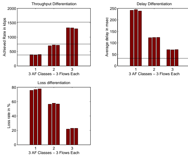
Figure 9. AHPD and CRED. Exponential traffic over UDP
