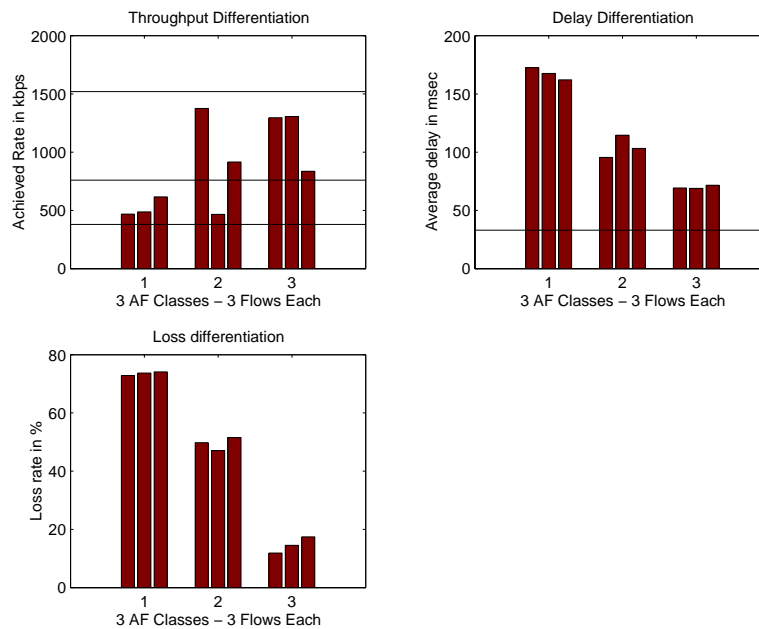
Figure 12. Original HPD: Pareto over UDP
