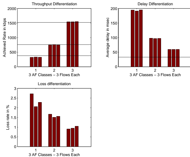
Figure 3. AHPD and CRED. FTP over TCP SACK. Bottleneck = 8 Mbps
