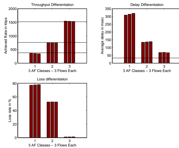
Figure 7. AHPD and CRED. All 9 flows are CBR/UDP
