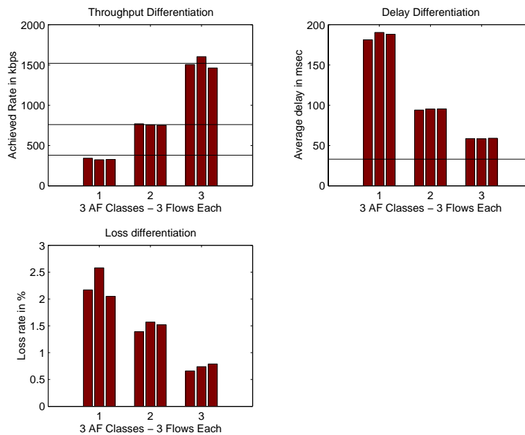
Figure 8. AHPD and CRED. Exponential traffic over SACK
