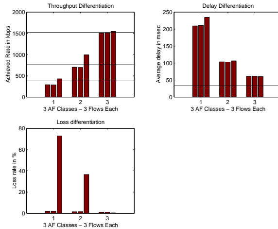
Figure 6. AHPD and CRED. Experiment with CBR. One flows in each class is CBR over UDP. Rest FTP/SACK
