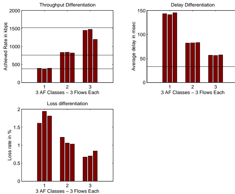
Figure 10. AHPD and CRED: Pareto over SACK
