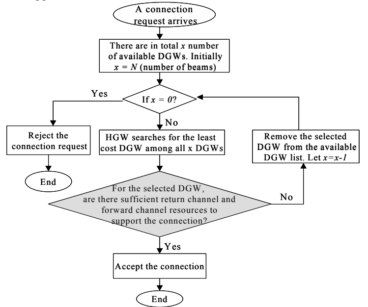
Figure 5. Proposed Call Admission Control flow chart in a satellite network with on-board cross-connect
