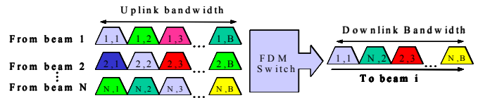
Figure 3. Return channel on-board connectivity
