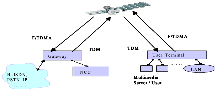
Figure 1. Network architecture for the Satellite network with on-board cross-connect
