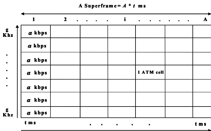
Figure 2. Return channel MF-TDMA frame structure
