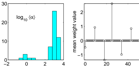
Figure 4: (Left) Histogram of the mean of the approximate \alpha posterior. (Right) A plot of the 51 (unthresholded) mean weight values (the first weight is the bias, the next 50 correspond to the 50 data points, read left-to-right, in Figure 3). The dichotomy into ‘relevant’ and ‘irrelevant’ weights is clear.
