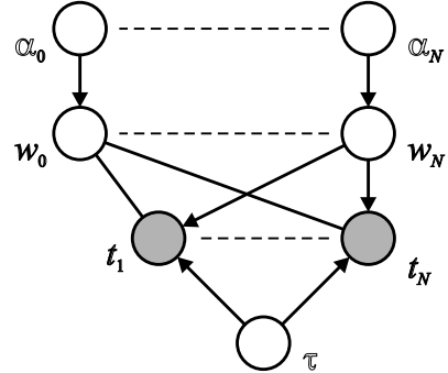
Figure 2: Directed acyclic graph representing the variational RVM as used for regression. The classification version is the same, with the omission of the \tau node.
