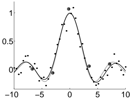
Figure 3: Example fit of a variational RVM to 50 data points generated from the ‘sinc’ function with added Gaussian noise of standard deviation 0.1. The sinc function and the mean interpolant are plotted in grey and black respectively, and the five relevance vectors (obtained by thresholding the mean weights at 10^{-3} ) are circled. The RMS deviation from the true function is 0.032, while a comparable SVM gave error of 0.038 using 36 support vectors. The VRVM also gives an estimate of the noise, which in this case had mean value 0.0945.
