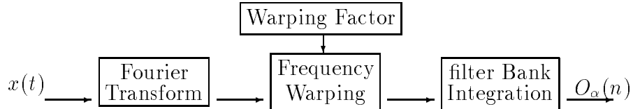
Figure 1: Frequency warping VTLN
