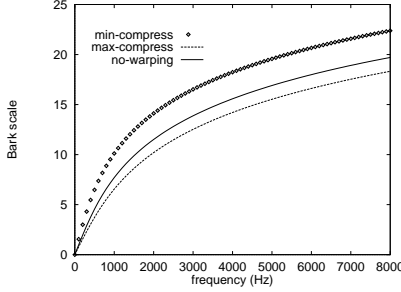
Figure 5: Bark scale warping curves
