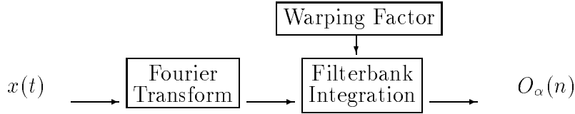
Figure 4: Speaker-specific Bark/Mel scale VTLN
