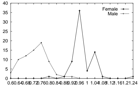
Figure 10: Histogram of Mel scale warping factors
