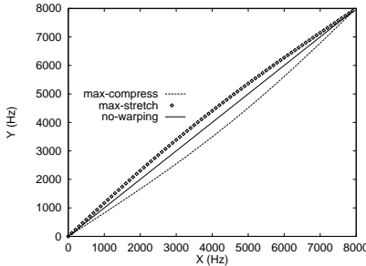
Figure 3: Bilinear warping curves
