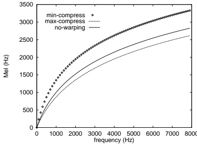
Figure 6: Mel scale warping curves
