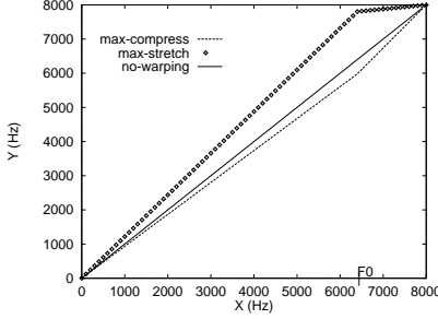
Figure 2: Piecewise warping curves
