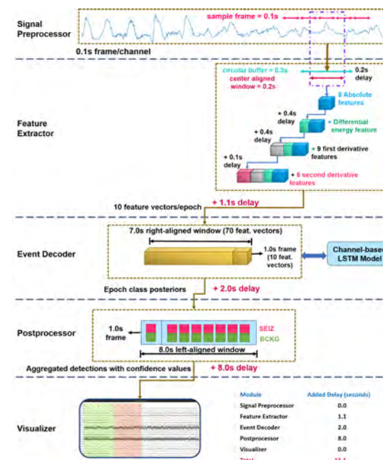
Figure 4: Data flow in the real-time system
