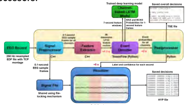
Figure 1. A block diagram of a real-time seizure detection system
