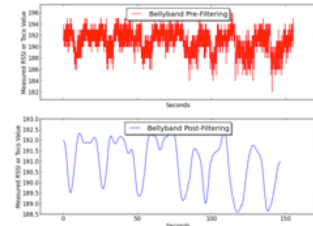
Fig. 2 - Bellyband RFID data is noisy and quantized, which is mitigated via the application of a Gaussian filter (bottom)
